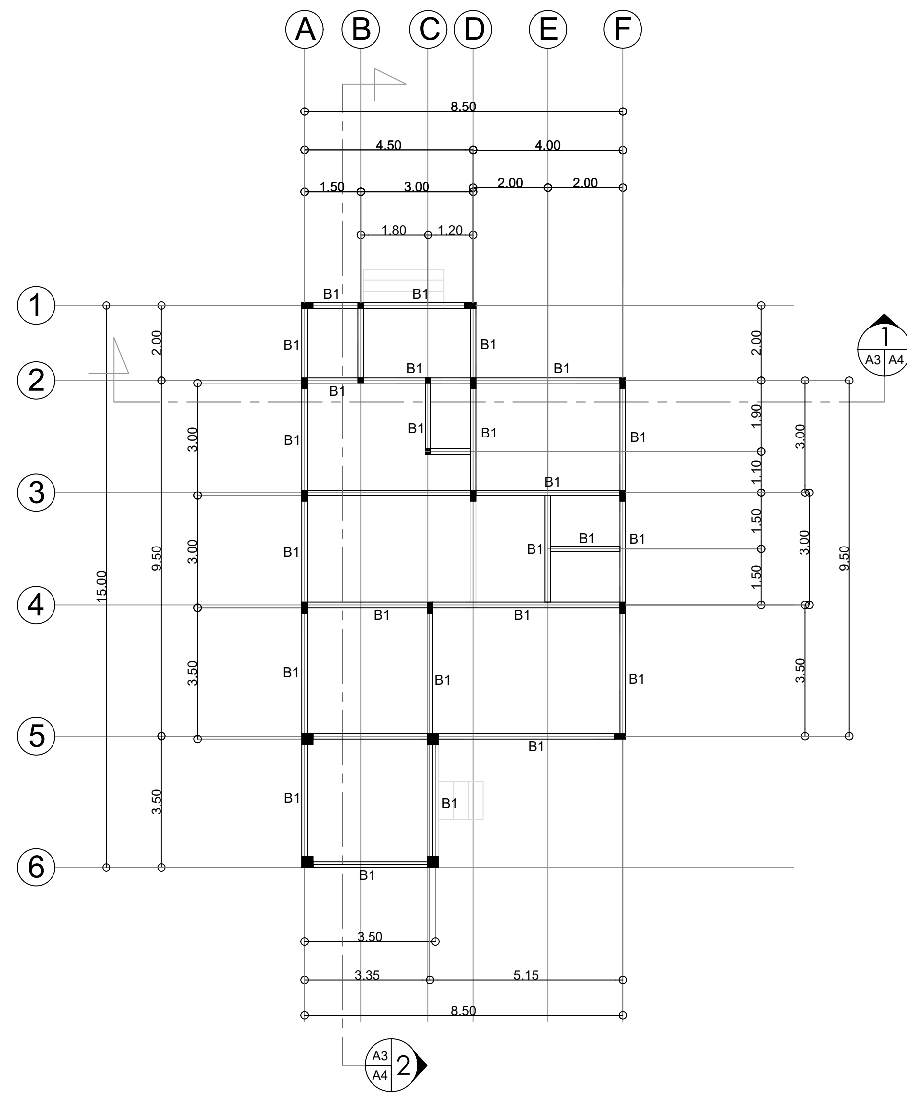
2 ROOF BEAM FRAMING PLAN SCALE 1 : 100 M.
