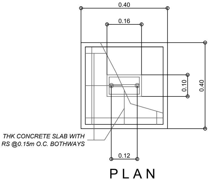
4 MANHOLE DETAILS P1 P1 SCALE 1 : 10 M.
