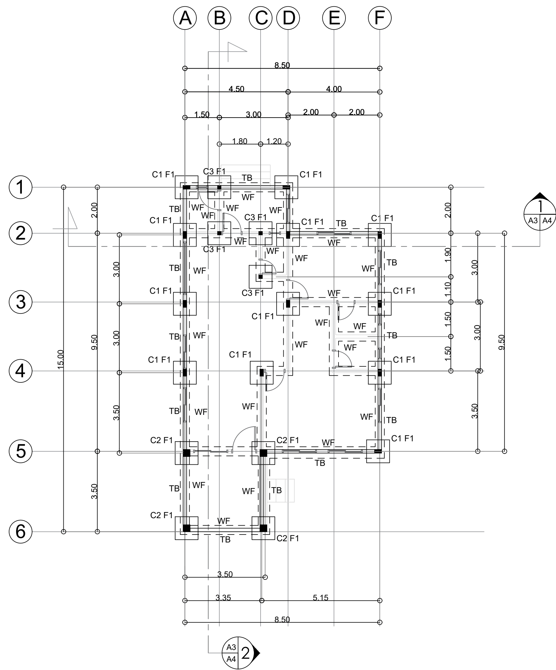
1 FOUNDATION PLAN SCALE 1 : 100 M.
