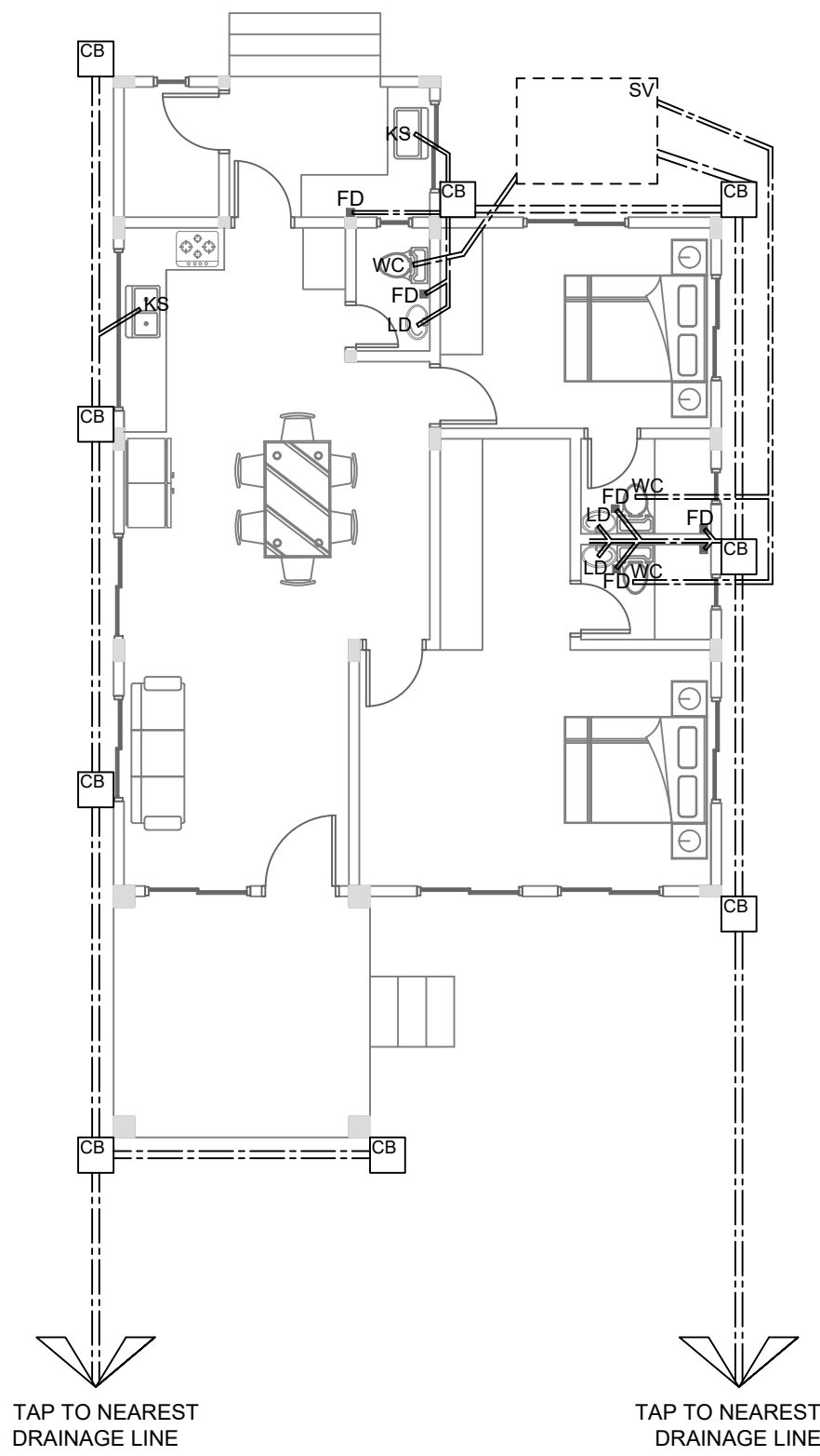
2 SANITARY LAYOUT P1 P1 SCALE 1 : 100 M.
