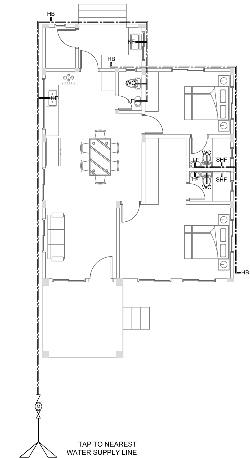
1 WATER DISTRIBUTION LAYOUT P1 P1 SCALE 1 : 100 M.
